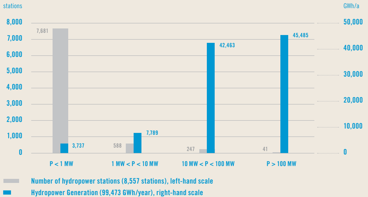
Contribution of different plant capacity categories to electricity generation from hydropower*
